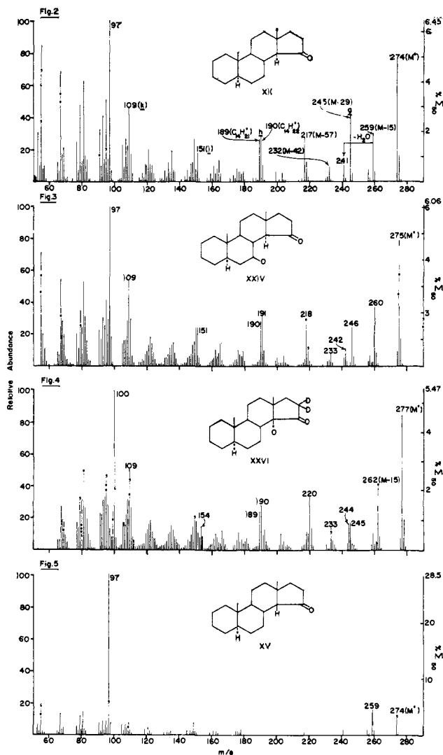
Figure 2. Mass spectrum of 5 \alpha -androstan-15-one (XII).
